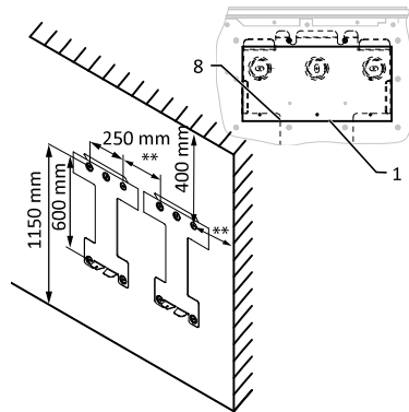
Fig. 14: Wall mounting
