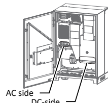
Fig. 7: Terminals
